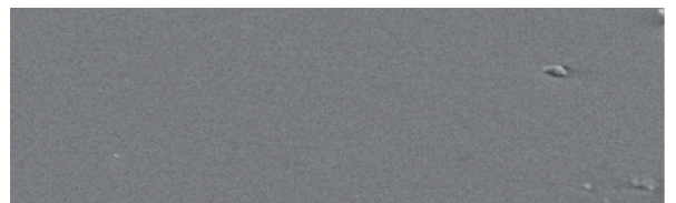
Magnified image of TIMELESS shower glass that has been in daily use: no rough whitish patches visible.
